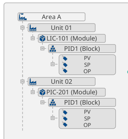
Plant A DeltaV Config
