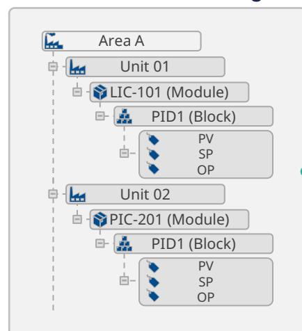
Plant B DeltaV Config
